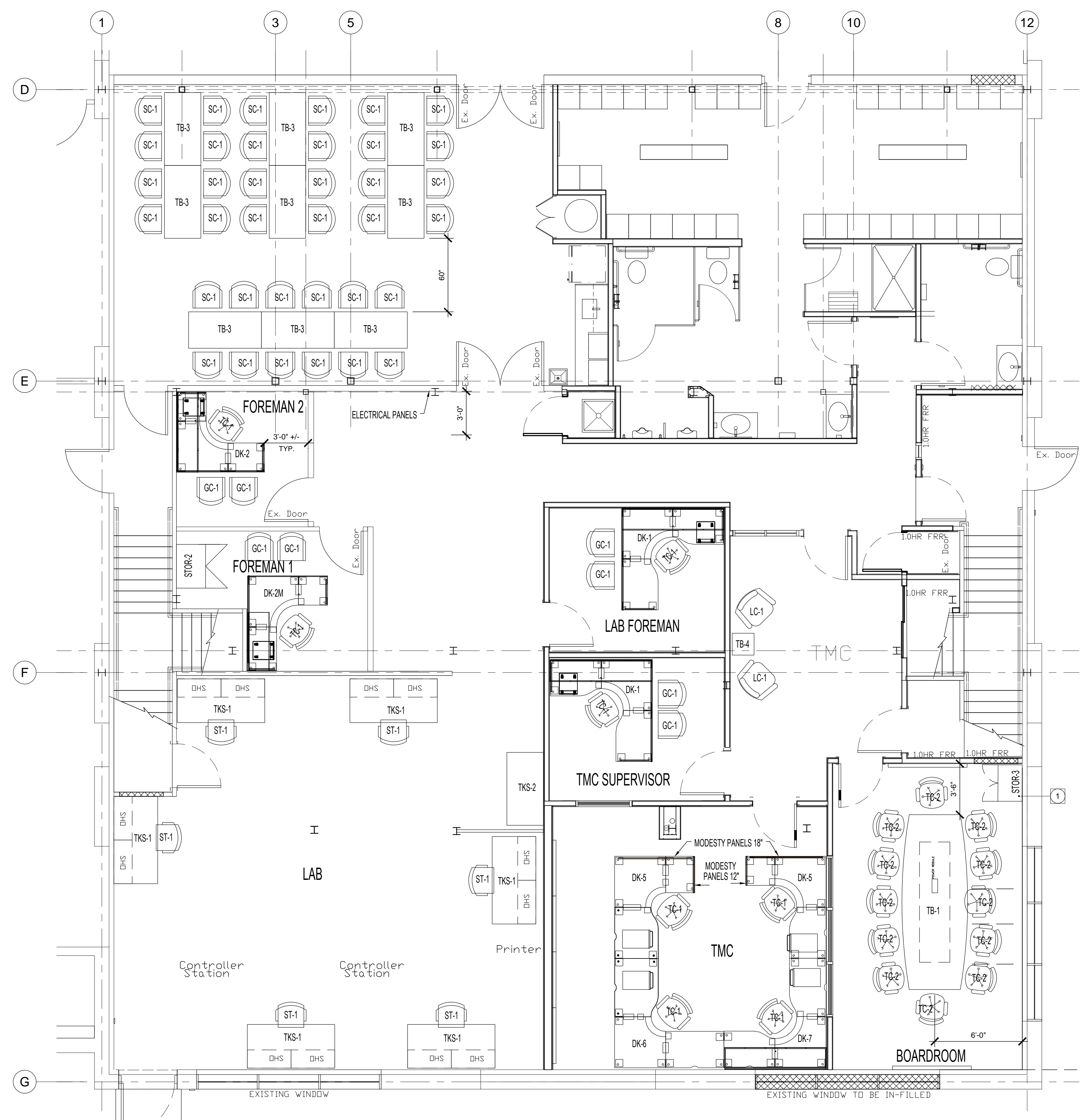
1 MAIN FLOOR FURNITURE PLAN SCALE: 1/4" = 1'-0"
